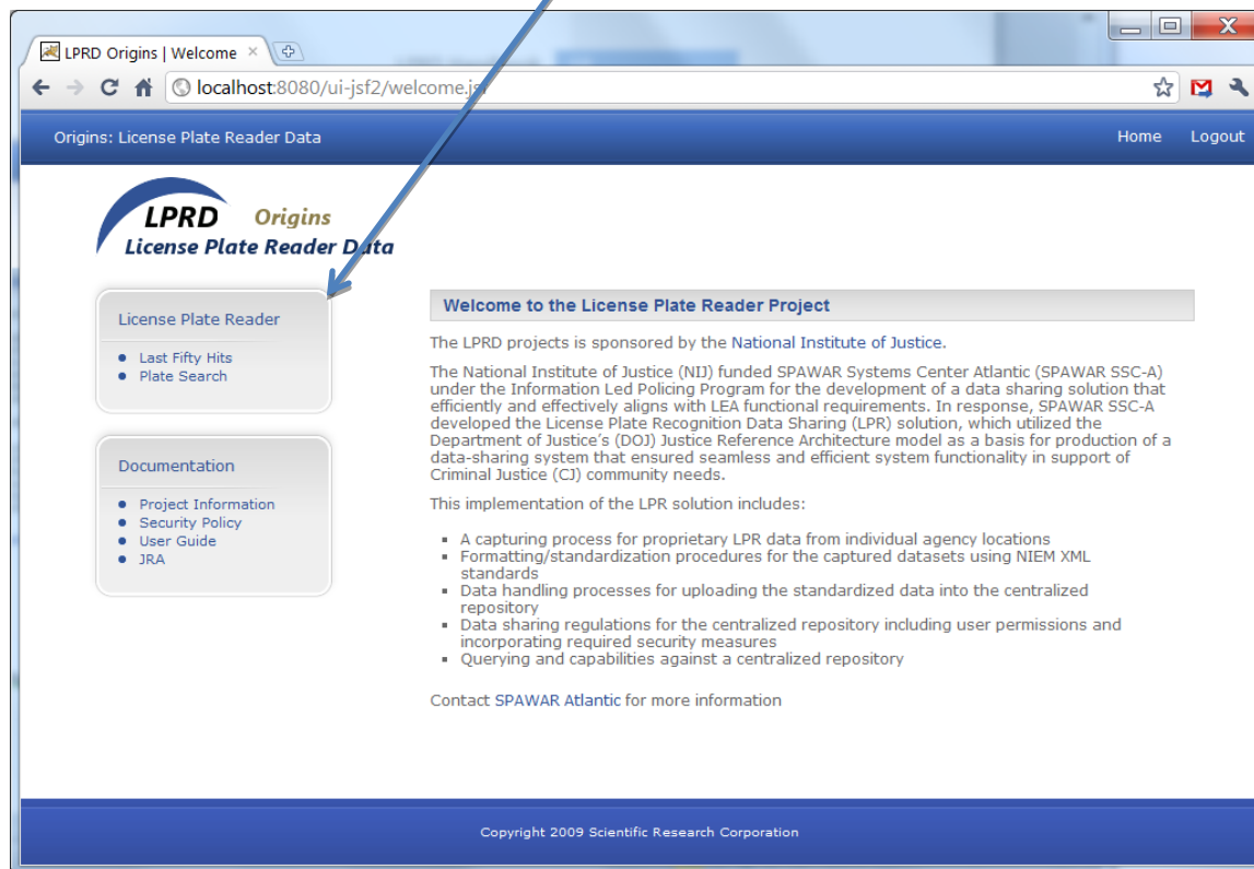
Figure 5 - LPR Header for an authenticated user
