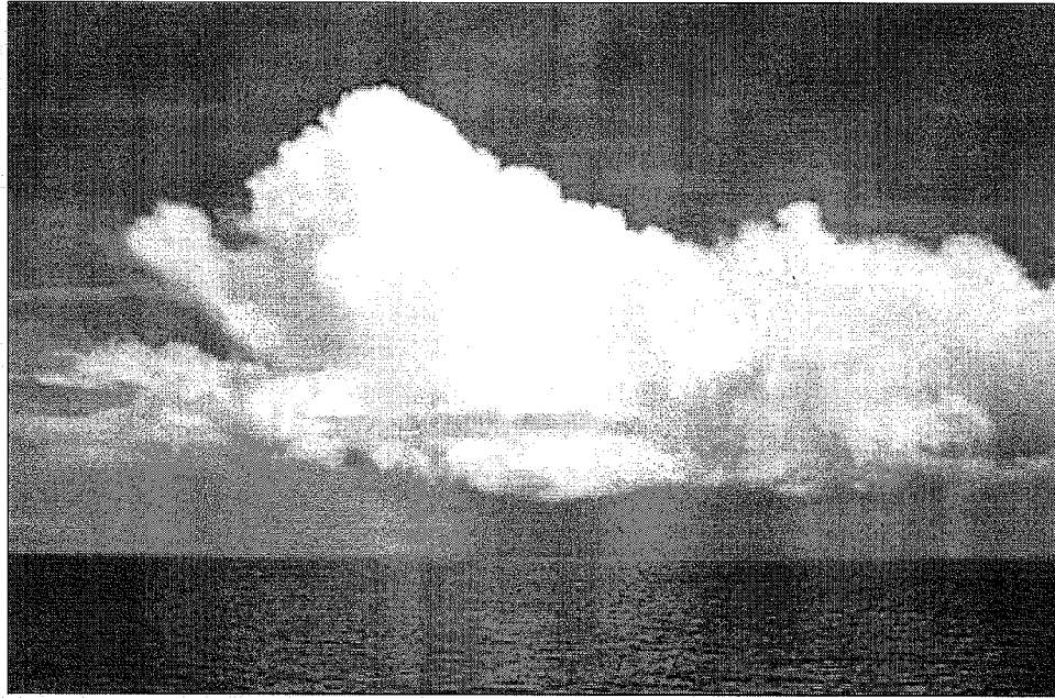
Figure 21: A cumulonimbus cloud. ( A Colour Guide to Clouds , Scorer and Wexler, p. 23.)
