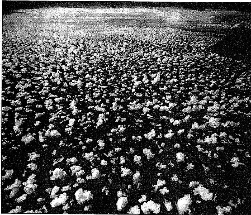
Figure 18: Small pieces of clouds (cumulus clouds) moving towards a convergence zone near the horizon, where we can see a large cumulonimbus cloud. ( Clouds and Storms , Ludlam, plate 7.4.)
