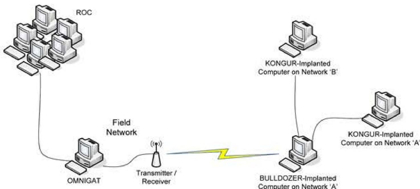
(TS//SI//REL) GINSU Extended Concept of Operations
