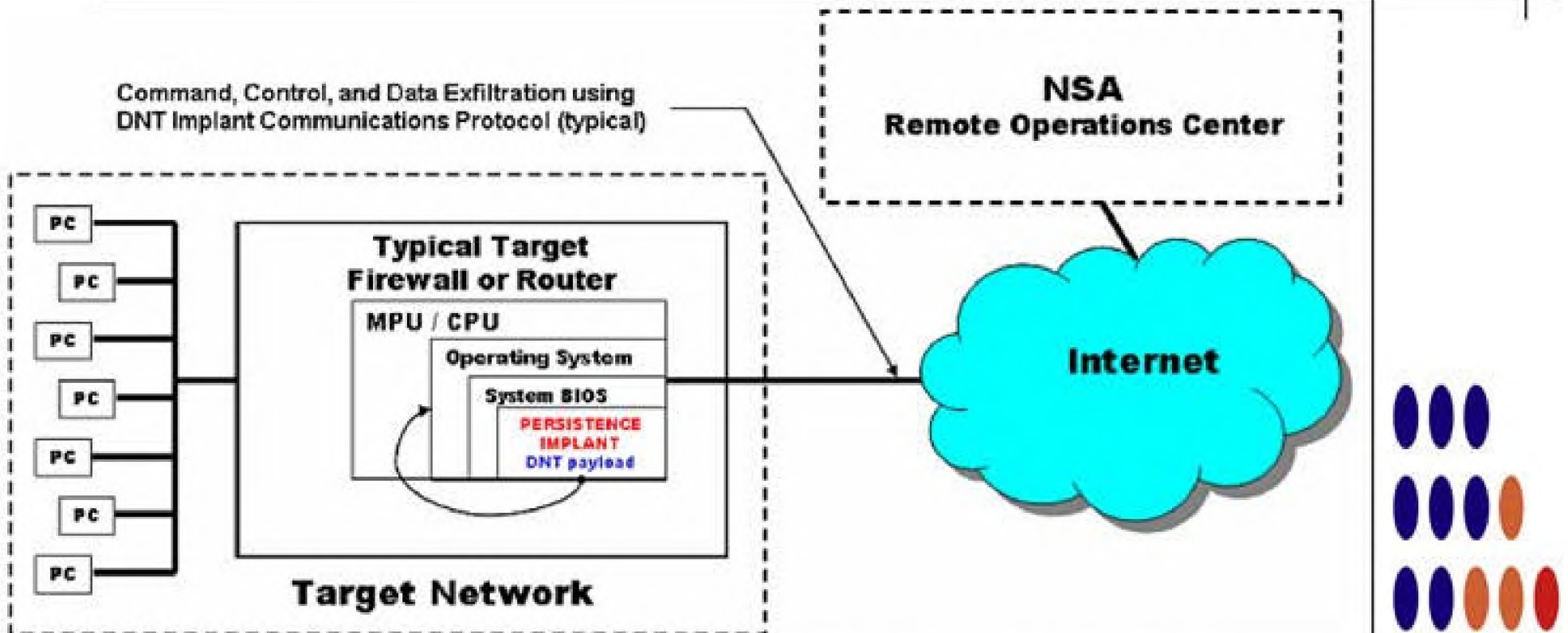
(TS//SI//REL) SOUFFLETROUGH Persistence Implant Concept of Operations
