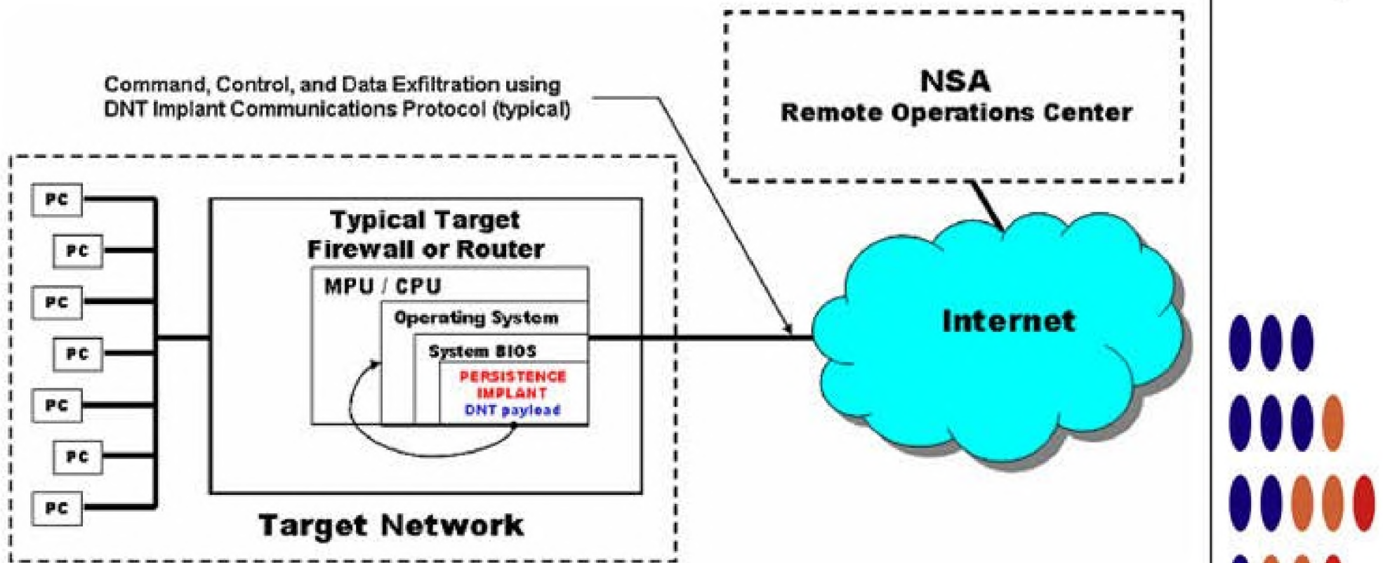
(TS//SI//REL) HALLUXWATER Persistence Implant Concept of Operations
