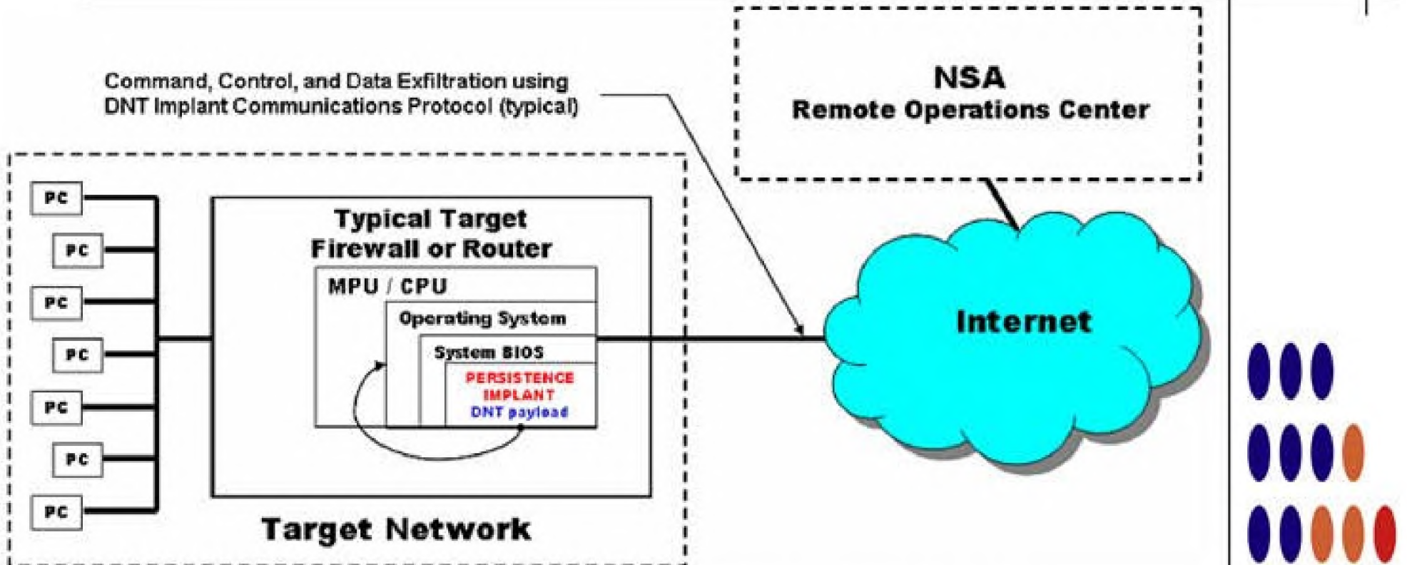
(TS//SI//REL) JETPLOW Persistence Implant Concept of Operations
